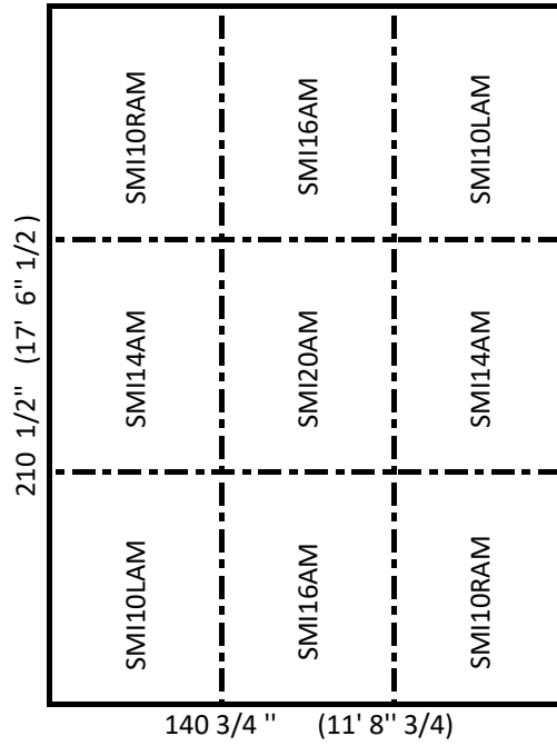
12 X 18 STALL
