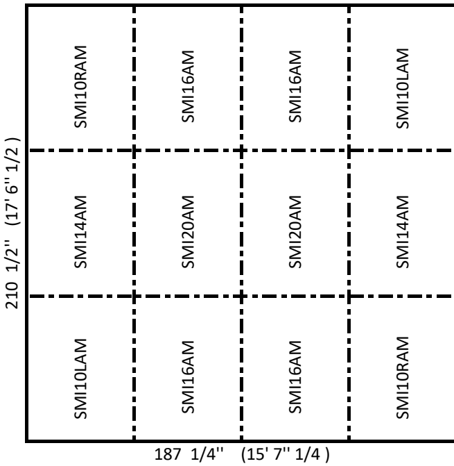
18 X 16 STALL
