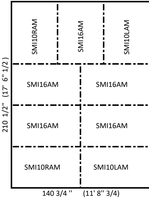
18 X 12 STALL
