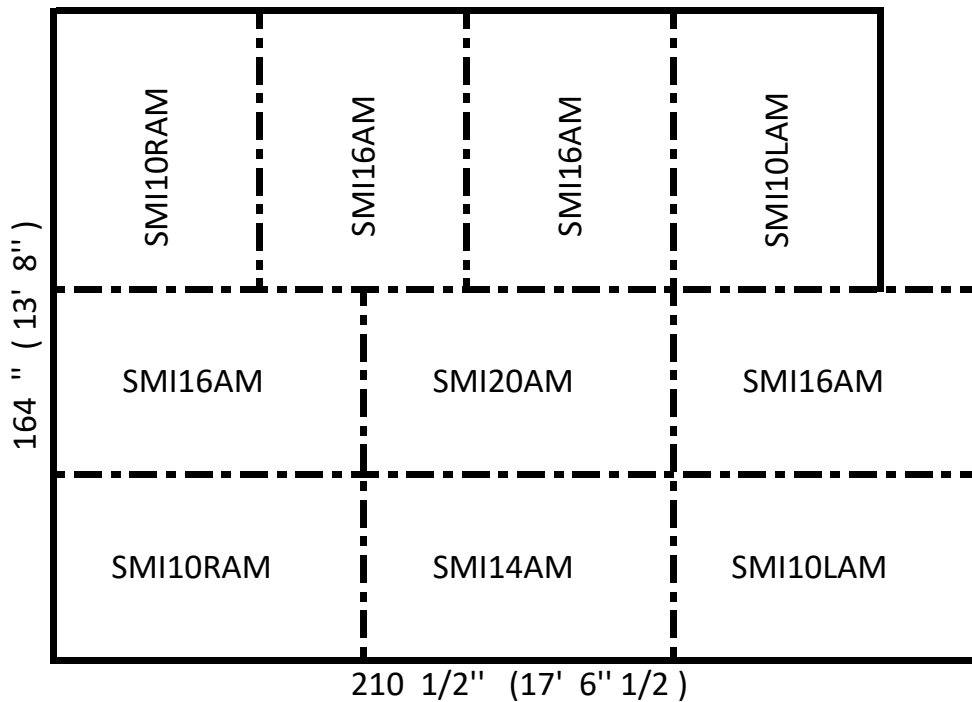
14 X 16 STALL
