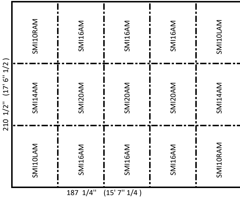
18 X 20 STALL
